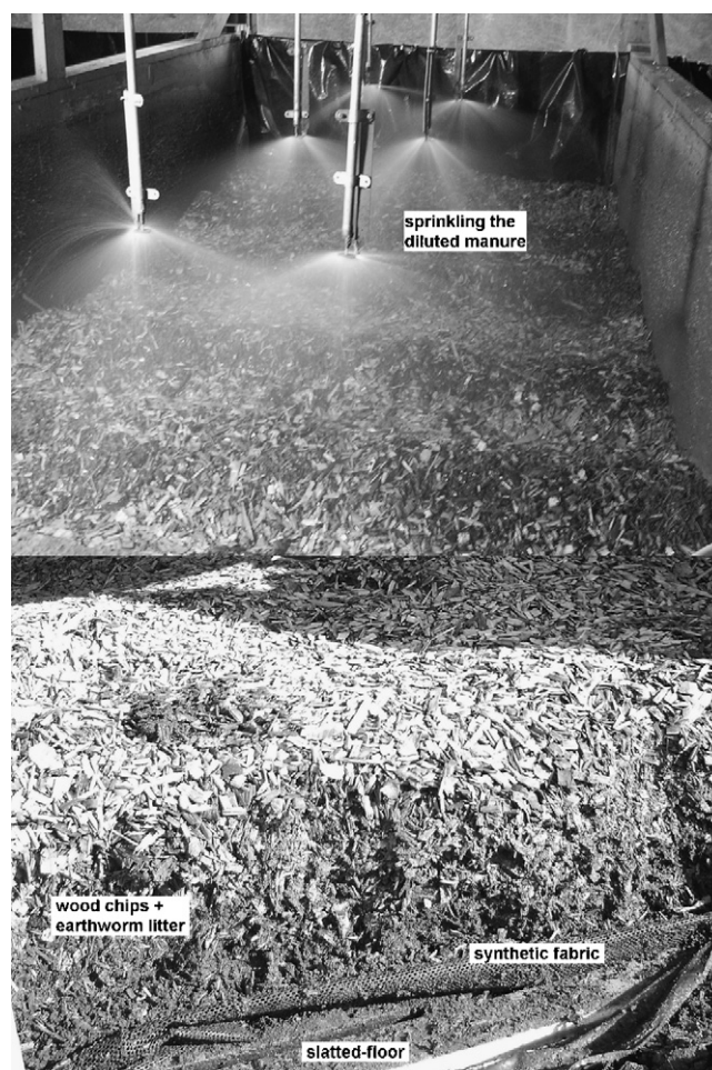
Fig. 1 – Photograph of the vermifilter.
